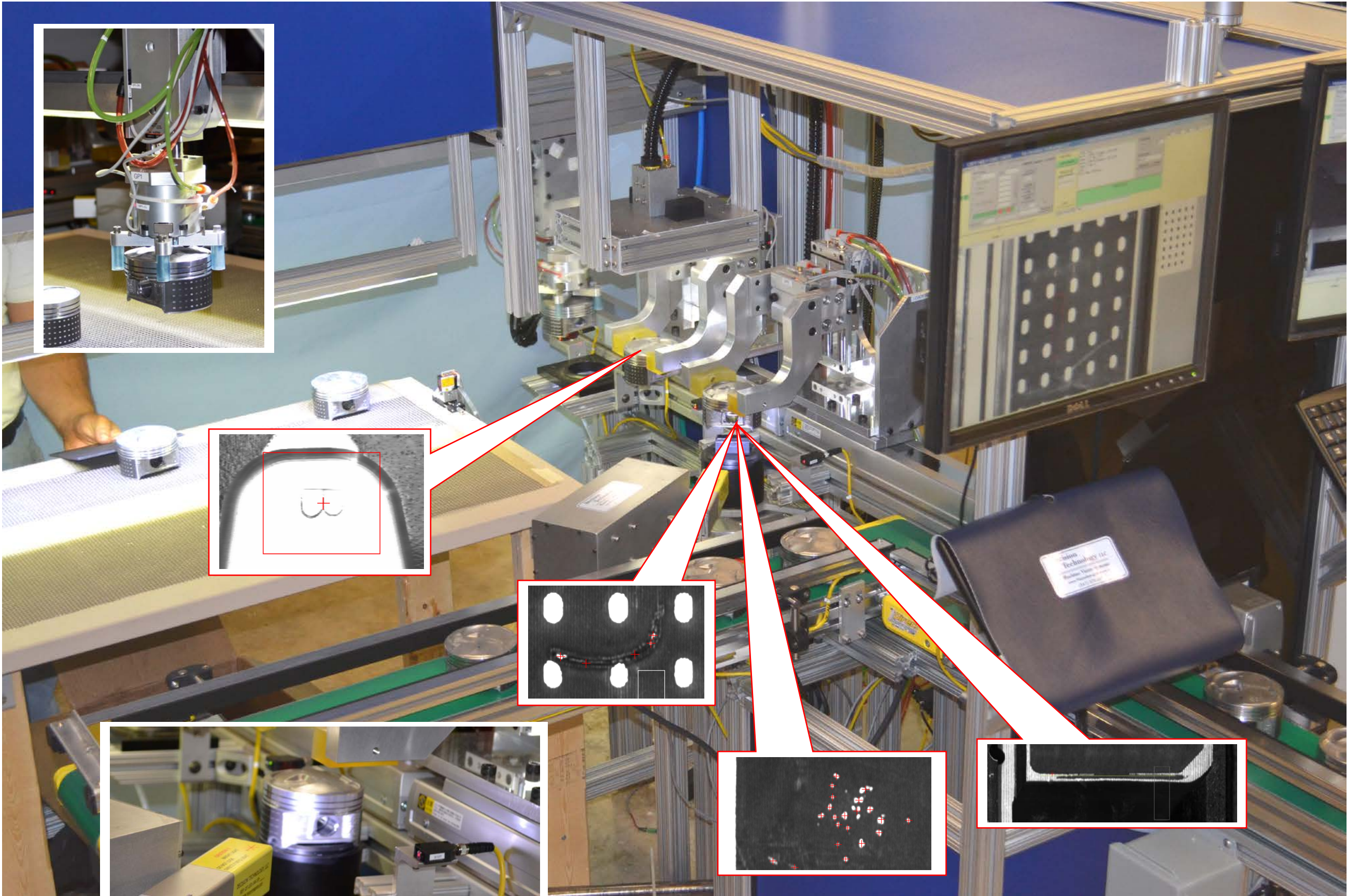
5 cameras: 2-part Guidance, 2-B & part # check, 1-Coating (line-scan) ~ 5 second cycle time
